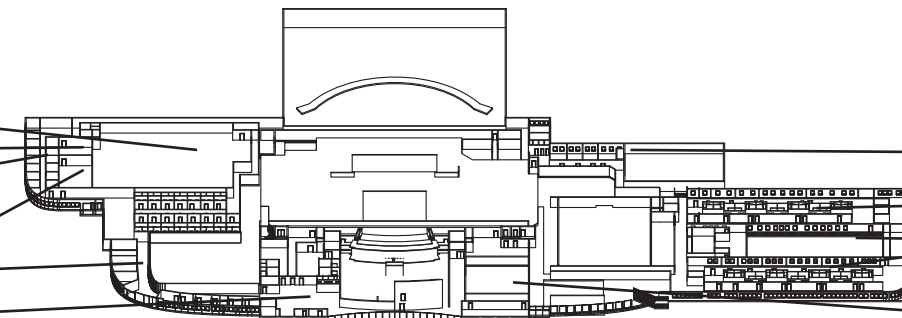
PLAN 3
